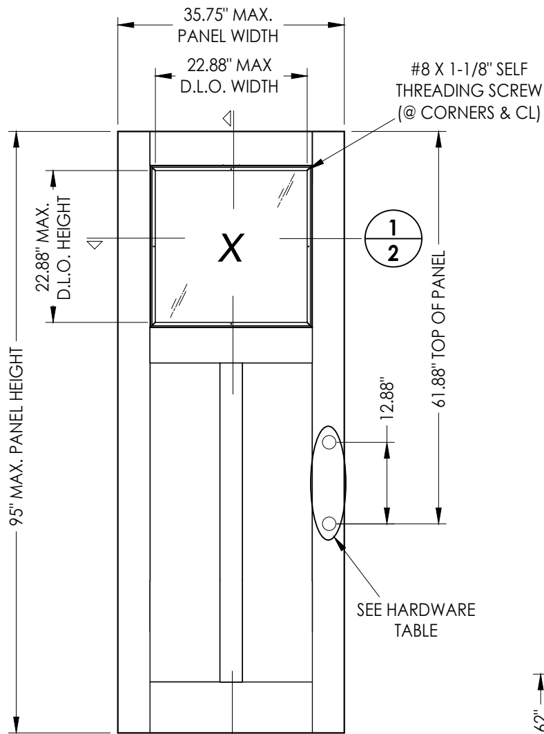
2 2 GLAZED DOOR PANEL LIGHHOUSE
