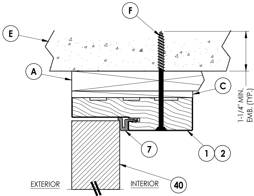
3 7 VERTICAL CROSS SECTION Outswing shown - Inswing also approved
