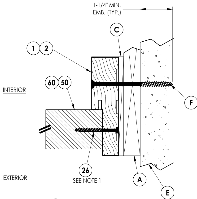
2 7 HORIZONTAL CROSS SECTION Outswing shown - Inswing also approved
